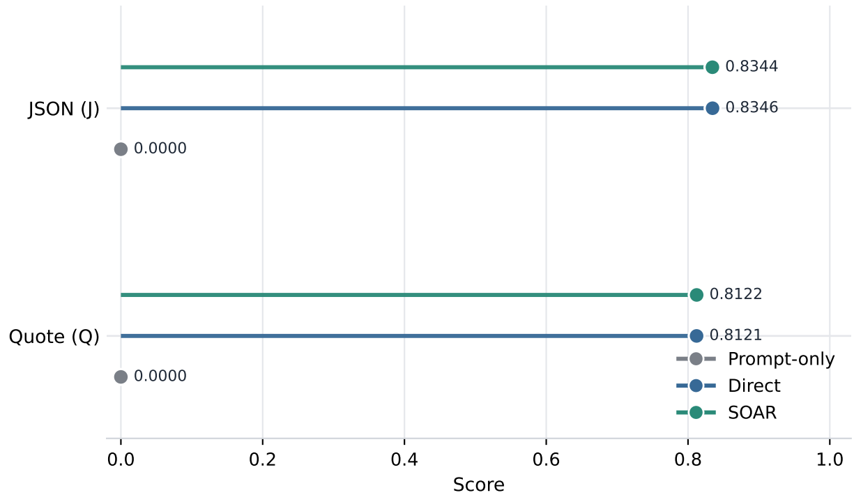
Answer F1 after parser extraction
