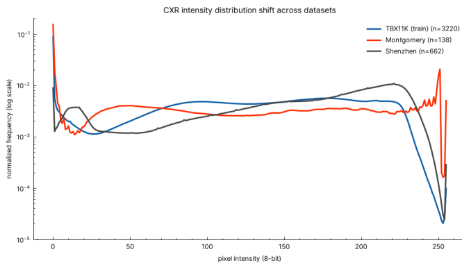
Fig. 6. Pixel-intensity distributions of the TBX11K training images and the two external sites. Montgomery is darker and Shenzhen brighter than the training set, the covariate shift in image appearance discussed in Section III-F that tracks the direction of the zero-shot failure on each site.
