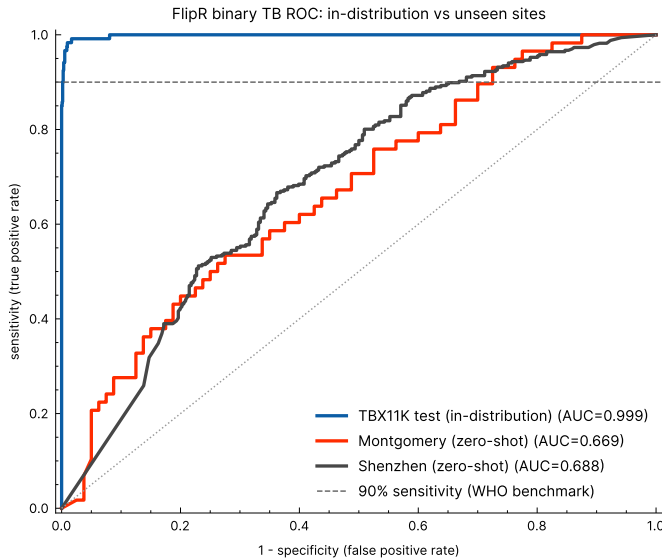
Fig. 3. Binary TB ROC for the FlipR classifier on the in-distribution TBX11K test set against the two unseen sites, Montgomery and Shenzhen. The in-distribution curve saturates in the top-left corner while both external curves fall toward the diagonal, showing the AUC collapse reported in Table III. The dashed line marks the 90% sensitivity operating point from WHO 2025 targets (minimum 40% specificity at 90% sensitivity) [7].
