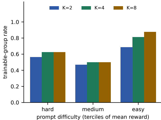
(b) trainable rate by difficulty
