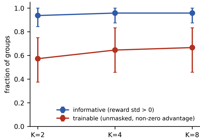
(a) informative vs trainable groups
