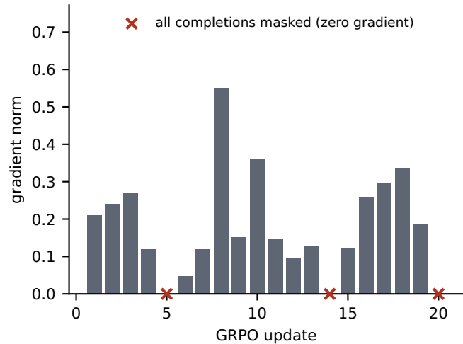
(c) standard run: gradient norm
