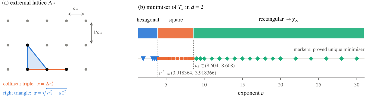
Fig. 1 (a) The extremal lattice \Lambda_* of Theorem 1: the collinear triple (red) and the right triangle (blue) have the same side-length product P_* . (b) Minimiser of T_\nu in d = 2 . Shaded regions: numerical phase diagram (Sect. 7); symbols: exponents at which the minimiser is established rigorously ( \nu = 2 classical, the others by Theorem 6). For \nu \rightarrow \infty the minimiser converges to \Lambda_* (Theorem 2).
