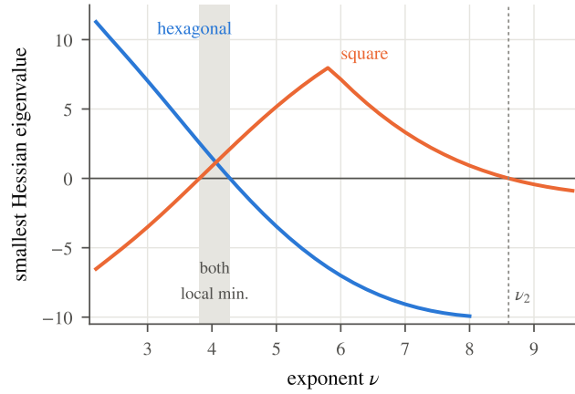
Fig. 4 Smallest Hessian eigenvalue of T_v at the hexagonal and at the square point. Grey: both are local minima, so the switch at \nu^* is discontinuous. Right: loss of stability of the square lattice at \nu_2 .
