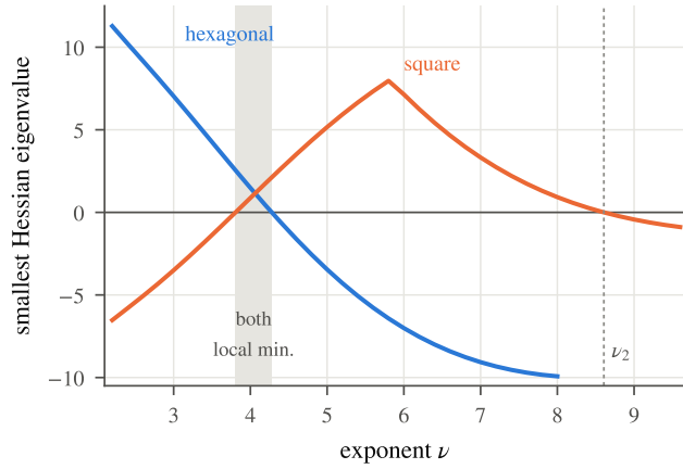
Fig. 3 Smallest Hessian eigenvalue of T_v at the hexagonal and at the square point. Grey: both are local minima, so the switch at \nu^* is discontinuous. Right: loss of stability of the square lattice at \nu_2 .
