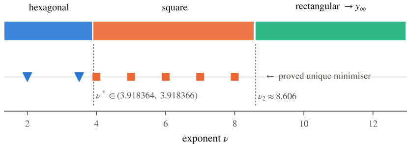
(b) minimiser of T_\nu in d = 2
