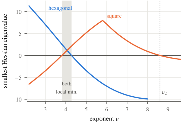
Fig. 4 Smallest Hessian eigenvalue of T_v at the hexagonal and at the square point. Grey: both are local minima, so the switch at v^* is discontinuous. Right: loss of stability of the square lattice at v_2 .
