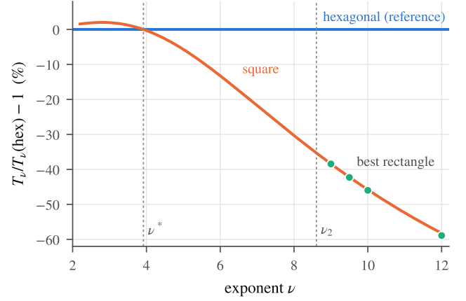
Fig. 3 Relative energy of the square lattice (line) and of the best rectangular lattice (dots) with respect to the hexagonal lattice. The zeros mark the switch at \nu^* and the bifurcation at \nu_2 .
