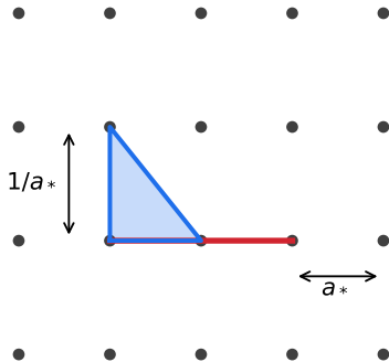
(a) extremal lattice \Lambda_* , 2a_*^3 = \sqrt{a_*^2 + a_*^{-2}}
