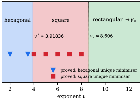
(b) phase sequence in d = 2
