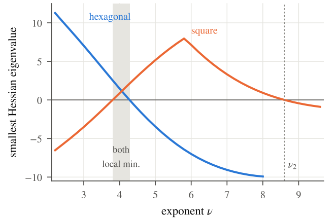
Fig. 4 Smallest Hessian eigenvalue of T_\nu at the hexagonal and at the square point. Grey: both are local minima, so the switch at \nu^* is discontinuous. Right: loss of stability of the square lattice at \nu_2 .
