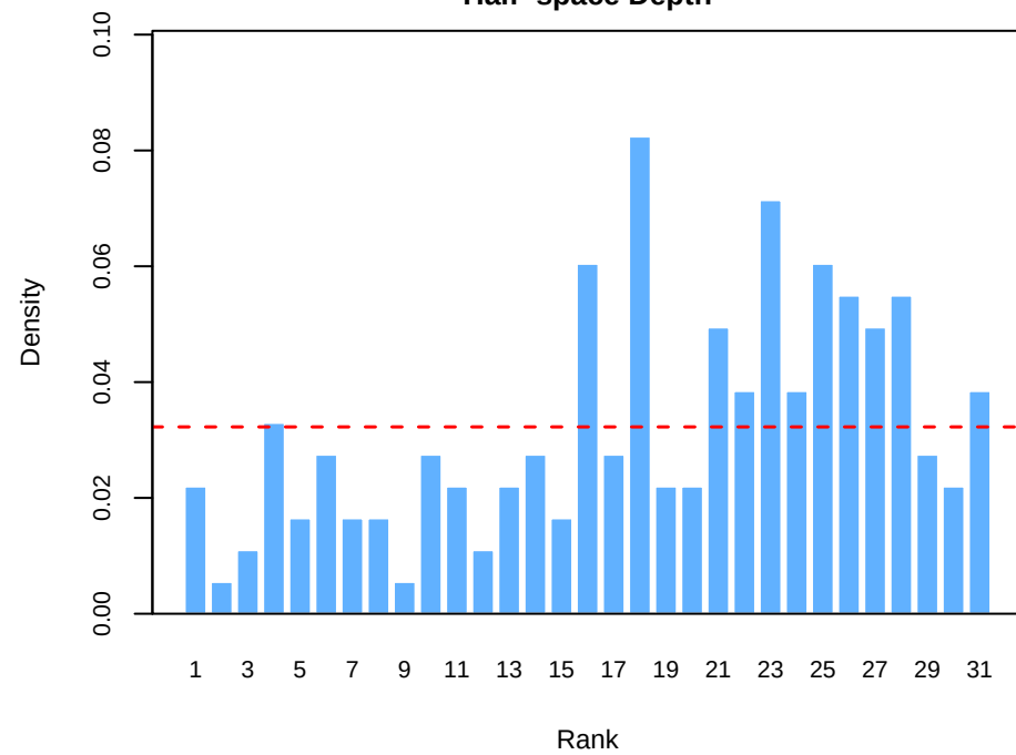
Half-space Depth
