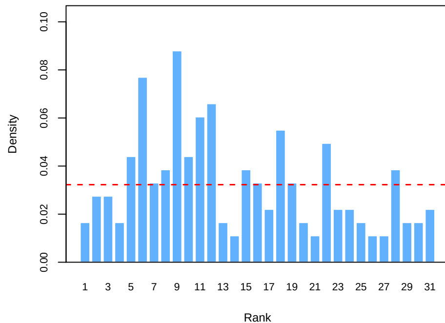
Half-space Depth
