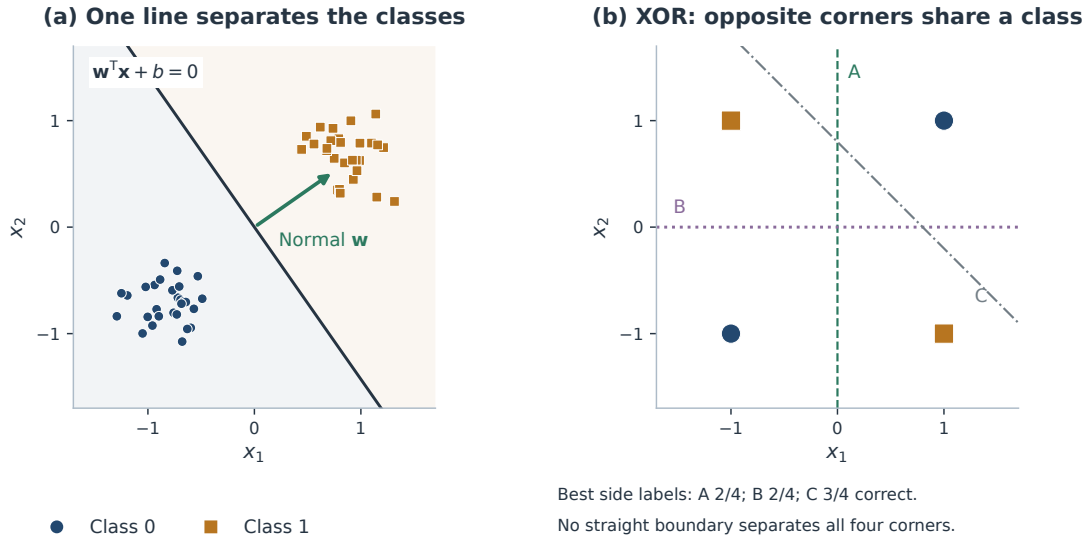
Figure 4.1: A linear classifier can separate two half-spaces with one flat boundary. Some class arrangements are not linearly separable, so no amount of optimisation can make one line solve them perfectly.
