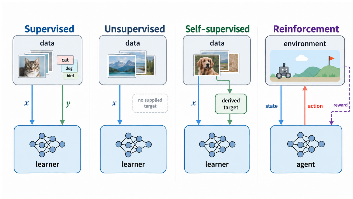
Figure 2.3: Learning paradigms differ mainly in the source and structure of the teaching signal. Modern systems often combine more than one paradigm.
