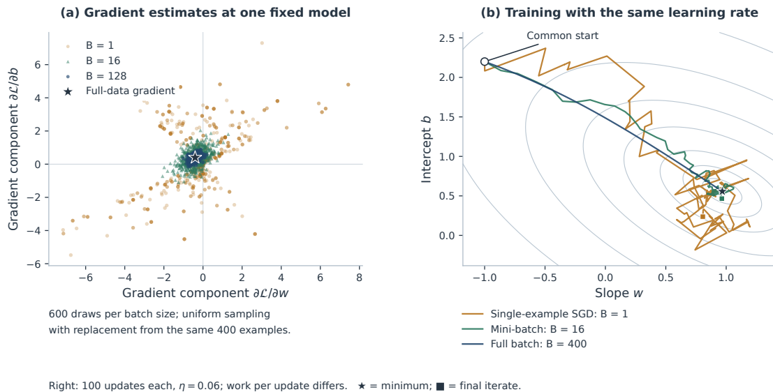
Figure 3.3: Mini-batch gradients are noisy estimates of the full-data gradient. Larger batches reduce variation, but a noisy trajectory can still make useful progress.
