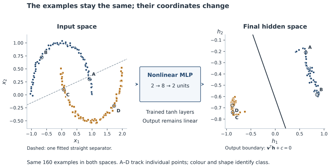
Figure 4.3: A hidden layer can reorganise the geometry of a problem. Here, the final two-unit hidden layer of a small MLP maps the same two-moons examples into new coordinates; letters track individual examples. The output layer remains linear in hidden space even though the corresponding decision boundary is nonlinear in the original input space.
