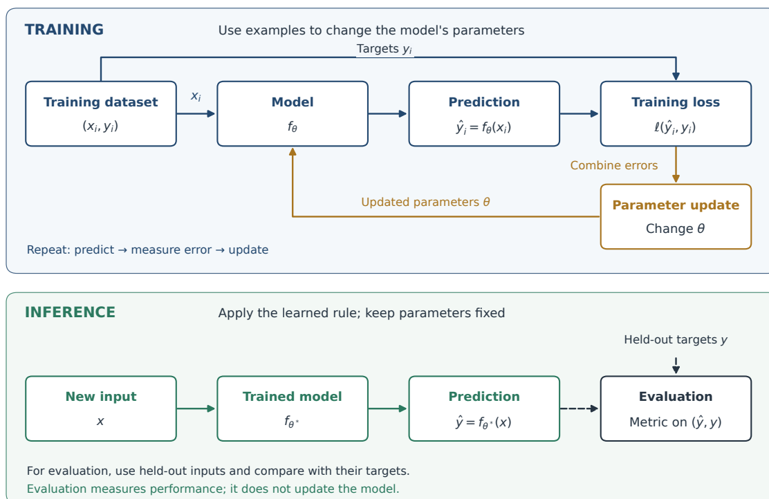
Figure 2.4: The skeleton of supervised learning. Week 1 names the parts; Week 2 will explain how the loss produces parameter updates.
