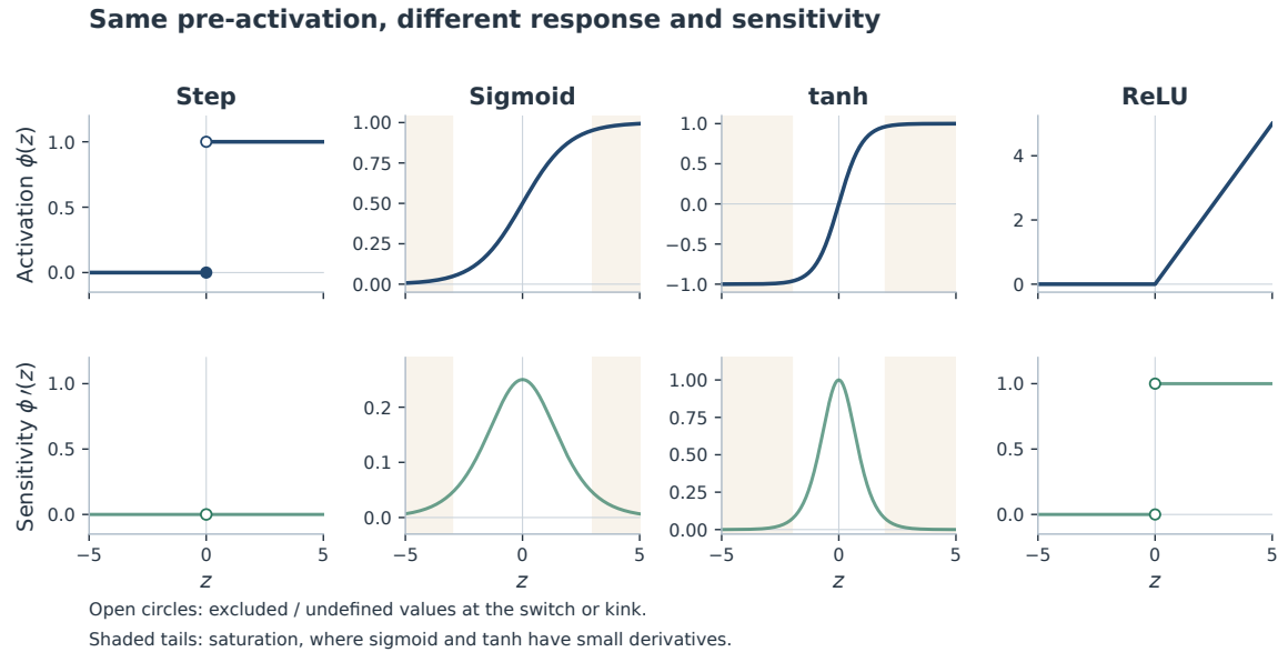
Figure 4.2: Common activation functions transform the same pre-activation in different ways. Their local sensitivities matter because gradients through a network are products of such local sensitivities.
