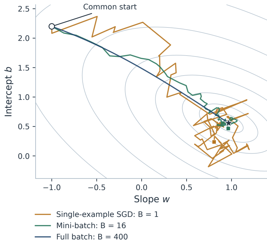
(b) Training with the same learning rate
