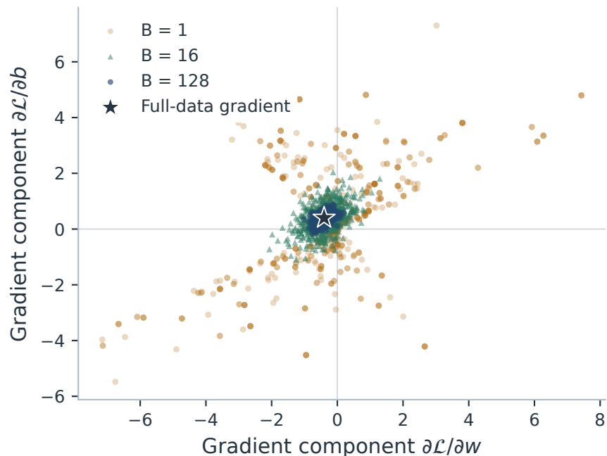
(a) Gradient estimates at one fixed model
