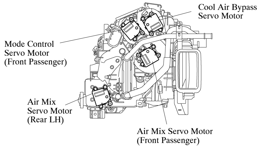
Front Air Conditioning Unit (LHD Models)
