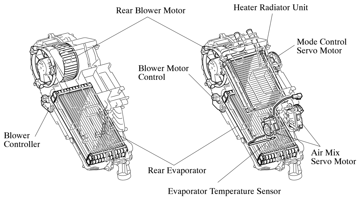
Models with Rear Cooler
