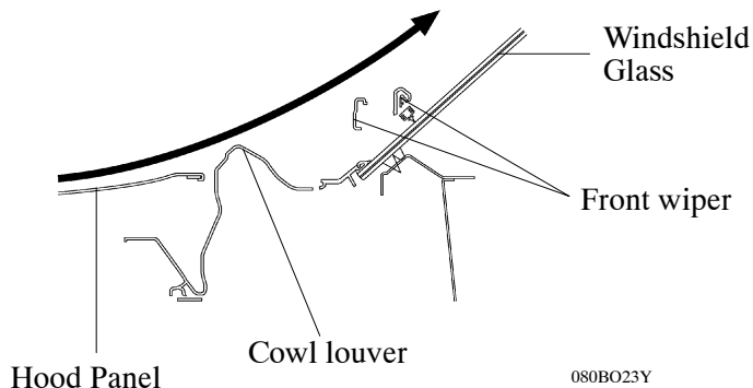
C-C cross section
