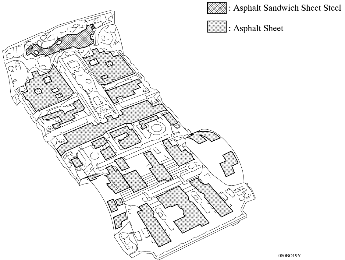
View from Top Side
