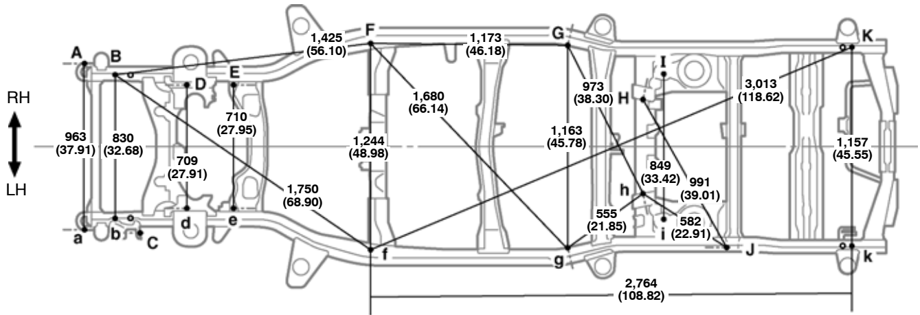
Vehicle Dimensions
