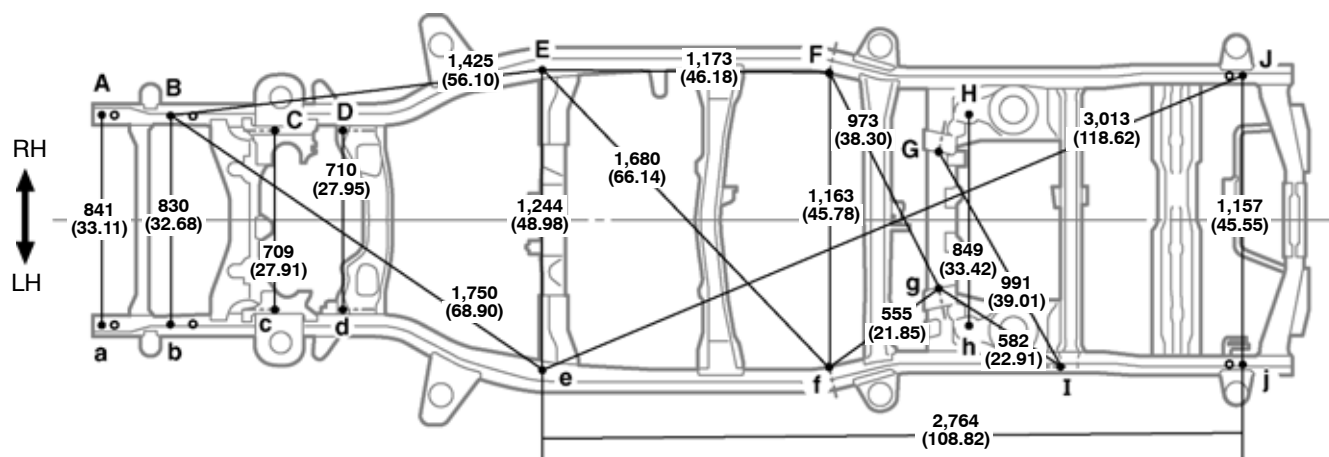
Vehicle Dimensions
