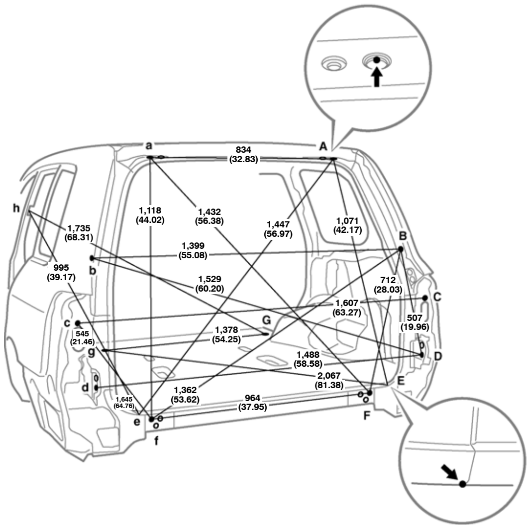
Vehicle Dimensions
