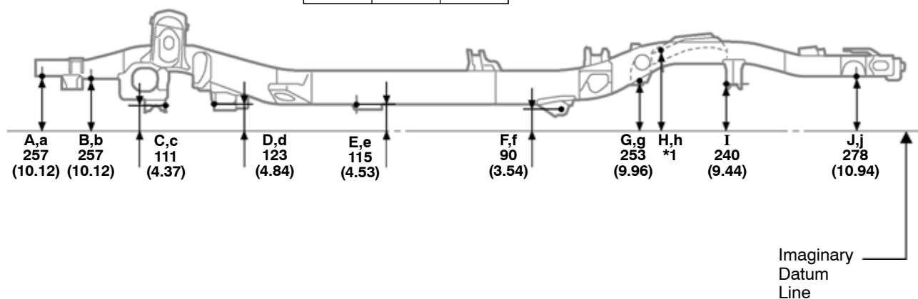
Vehicle Dimensions
