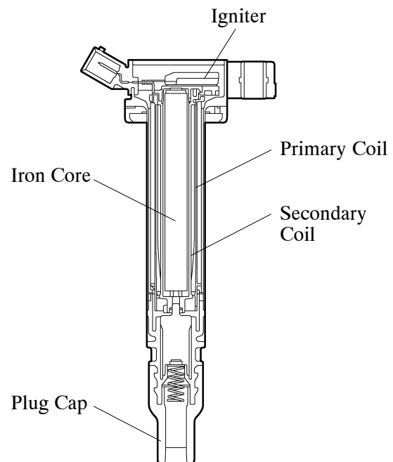
Ignition Coil Cross Section
