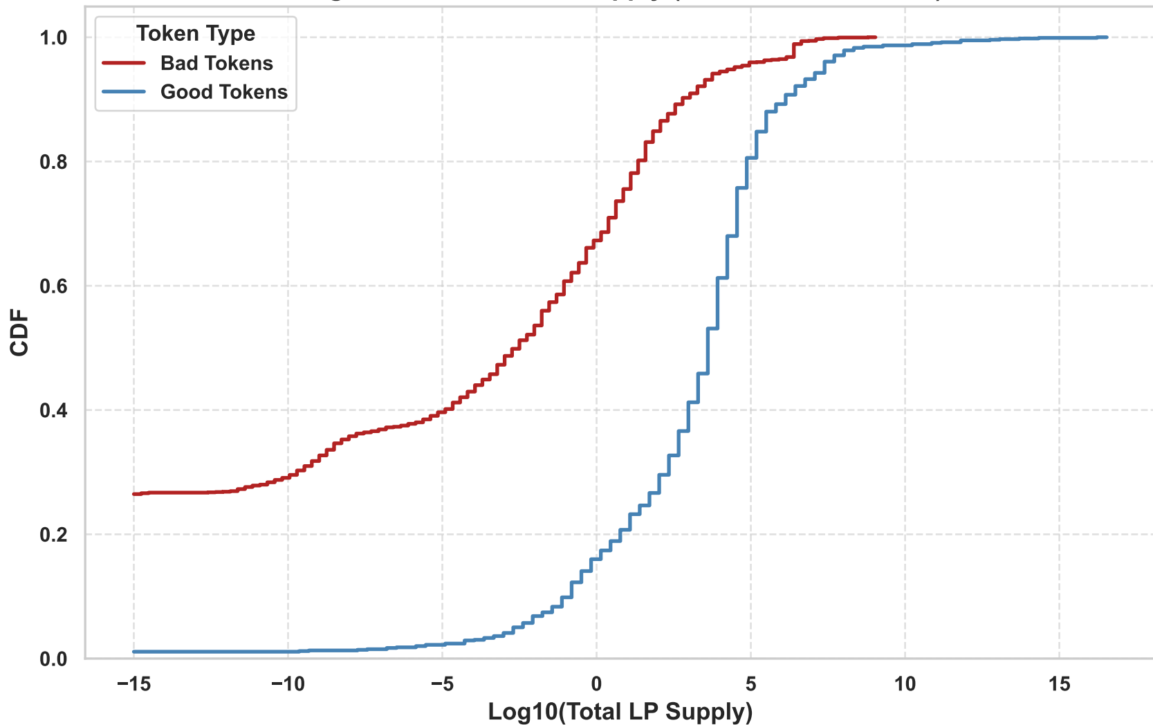
Log10 CDF of Total LP Supply (Good vs Bad Tokens)
