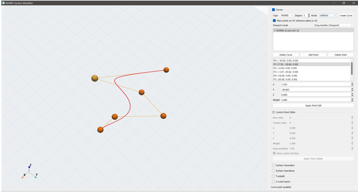
Figure 2: GUI interface for curve creation and manipulation. Shows the viewport with rendered curve and control points, alongside the Curves Panel with type selector, degree spinner, and control point list editor.
