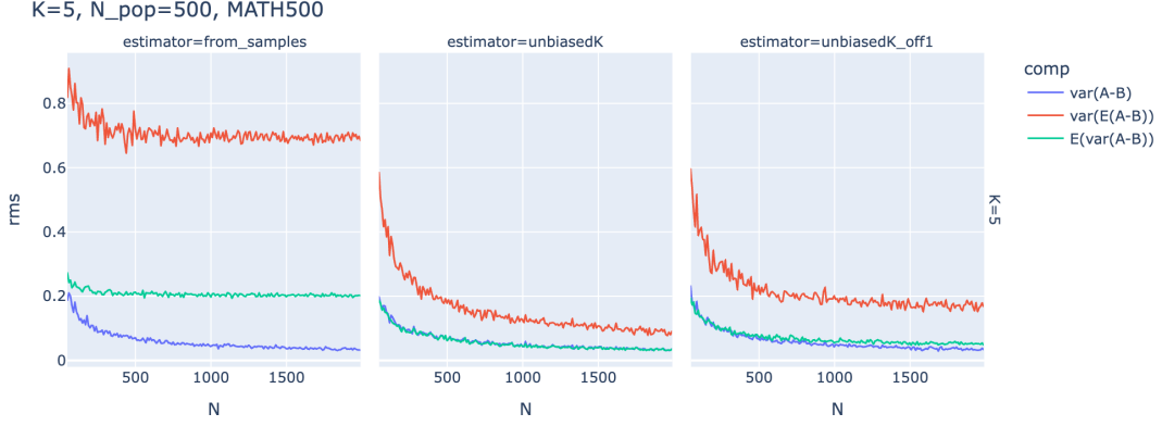
Figure 3: Relative errors of the paired noises. The left figure without the correction on K has an unacceptably high 70% relative error even with 2000 data points. 1000 predictions are drawn from model A and B on each of 500 questions of MATH500, which is treated as the ground truth. K = 5 samples are drawn from the 500 samples and the root mean squared relative errors of variance components are plotted vs. bootstrap sample size N , which extends beyond the population size 500.
