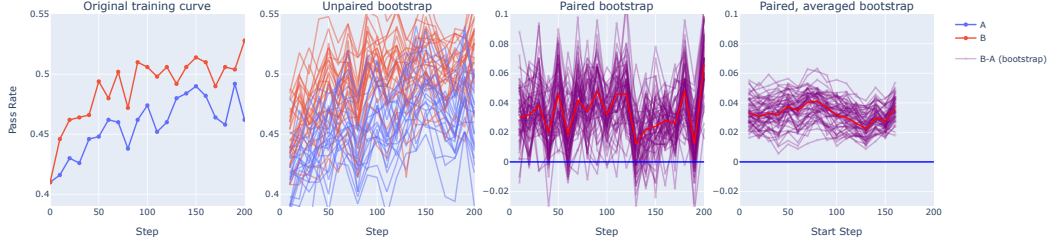
Figure 2: Column 1) The original training curve where A and B both starts from the same checkpoint at step 0 where data noise is 0. 2) Under the unpaired bootstrap data noise, many baselines A is higher than B, showing a meaningless difference. 3) Some significance with a z -score of 1.7 with the paired bootstrap at 1 prediction per question. 4) The result is very significant with a z -score of 3.5 if we average over 5 consecutive training checkpoints and reduce the prediction noise.
