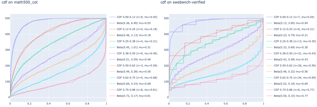
Figure 6: Empirical cummulative distribution curves (CDF, solid) and their respective Beta models (dots). Each color represents a different bin by model accuracy. The average accuracy of each question in each bin of models is computed and sorted to produce the CDF curves. The fit is good.
