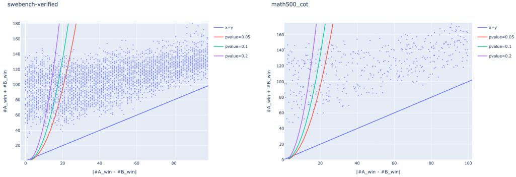
Figure 7: The amount of inconsistency.
