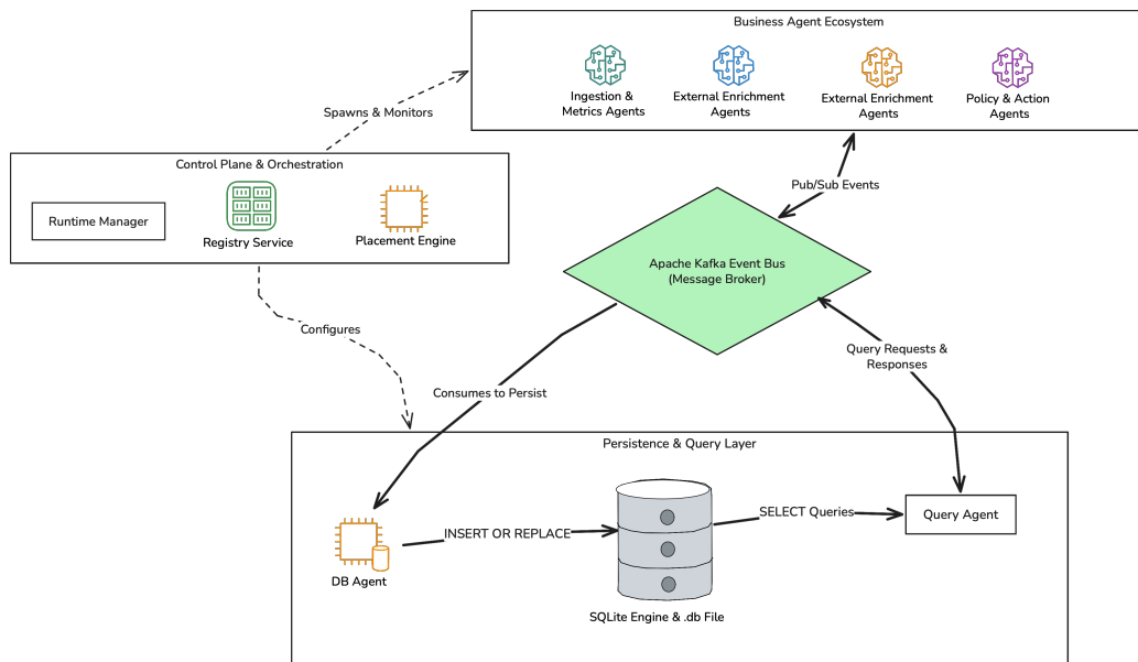
Fig. 5.2 Component design of ACIS-X
