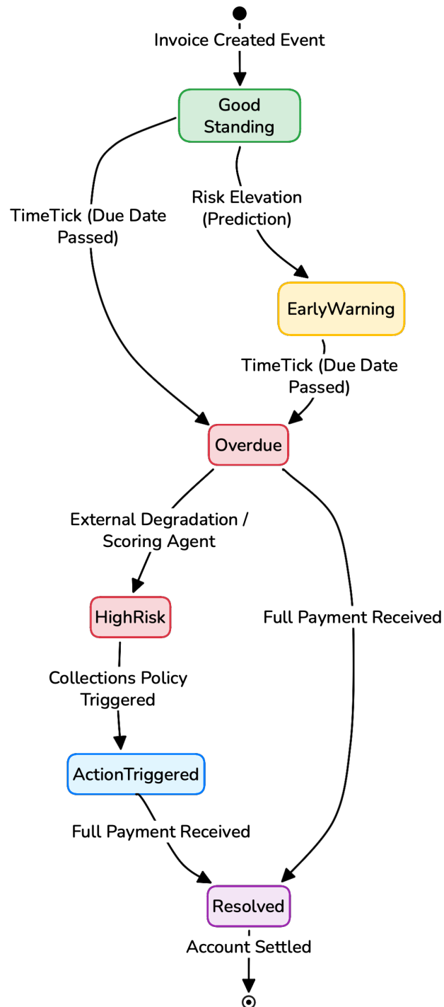
Fig. 3.4 State chart diagram specifying account state transitions
