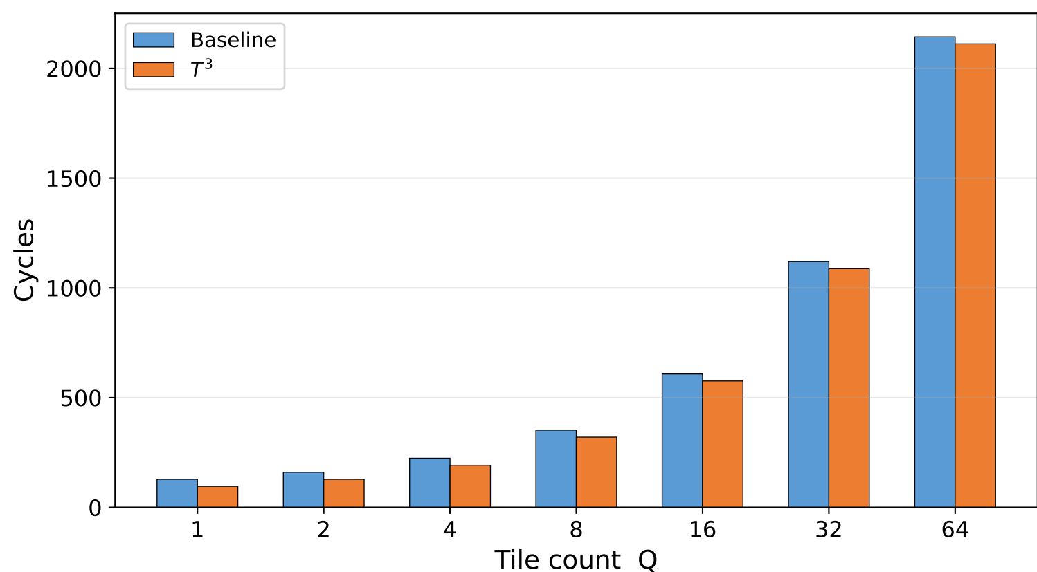
(a) Cycle Count at M/D=1
