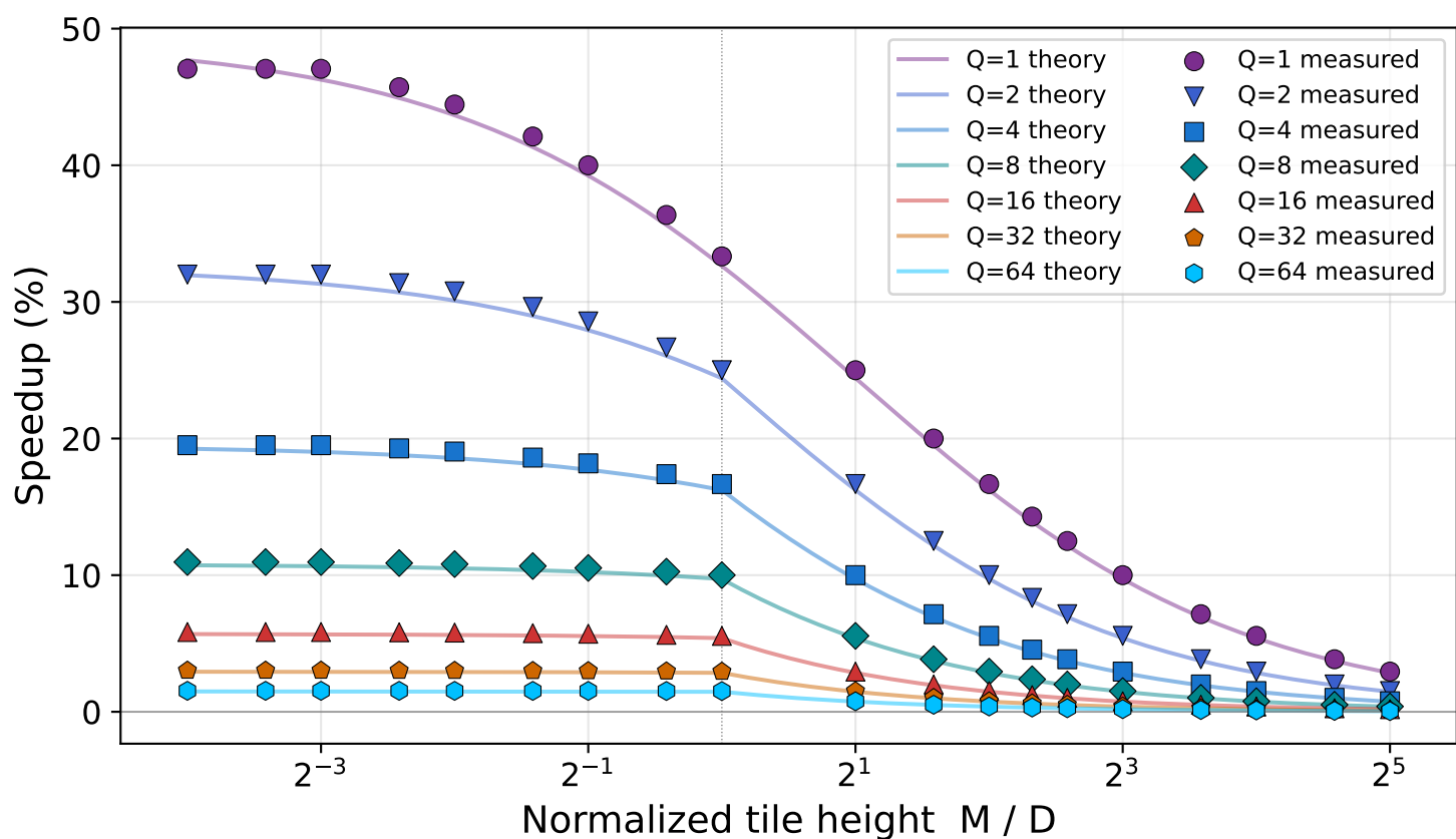
(b) Gemmini Single-GEMM T^3 Compute-Only Speedup
