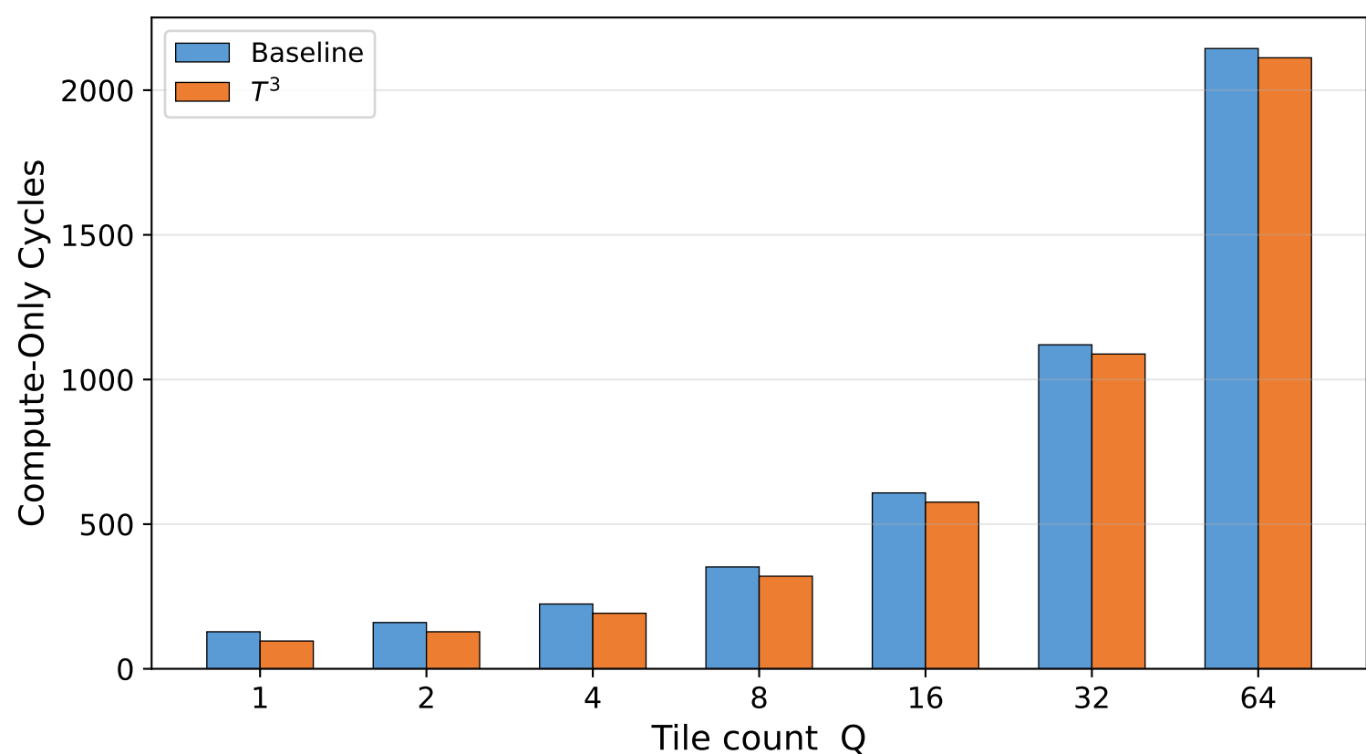
(a) Compute-Only Cycles at M/D=1
