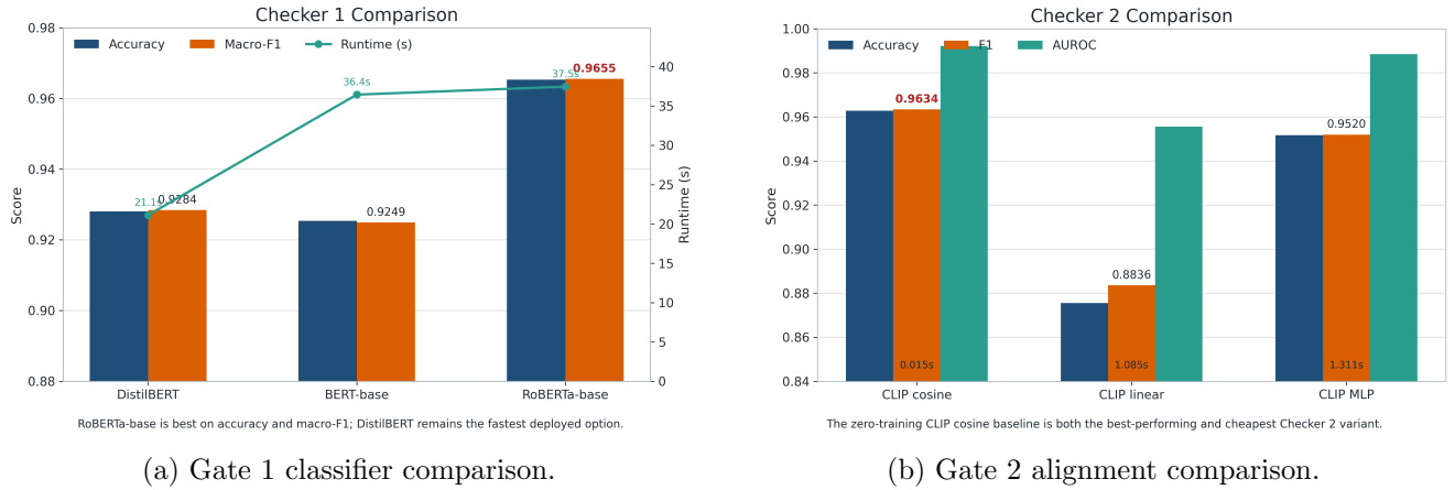
Figure 7: Offline experiment figures generated from saved experiment records. These plots do not show live request latency or learning outcomes.
