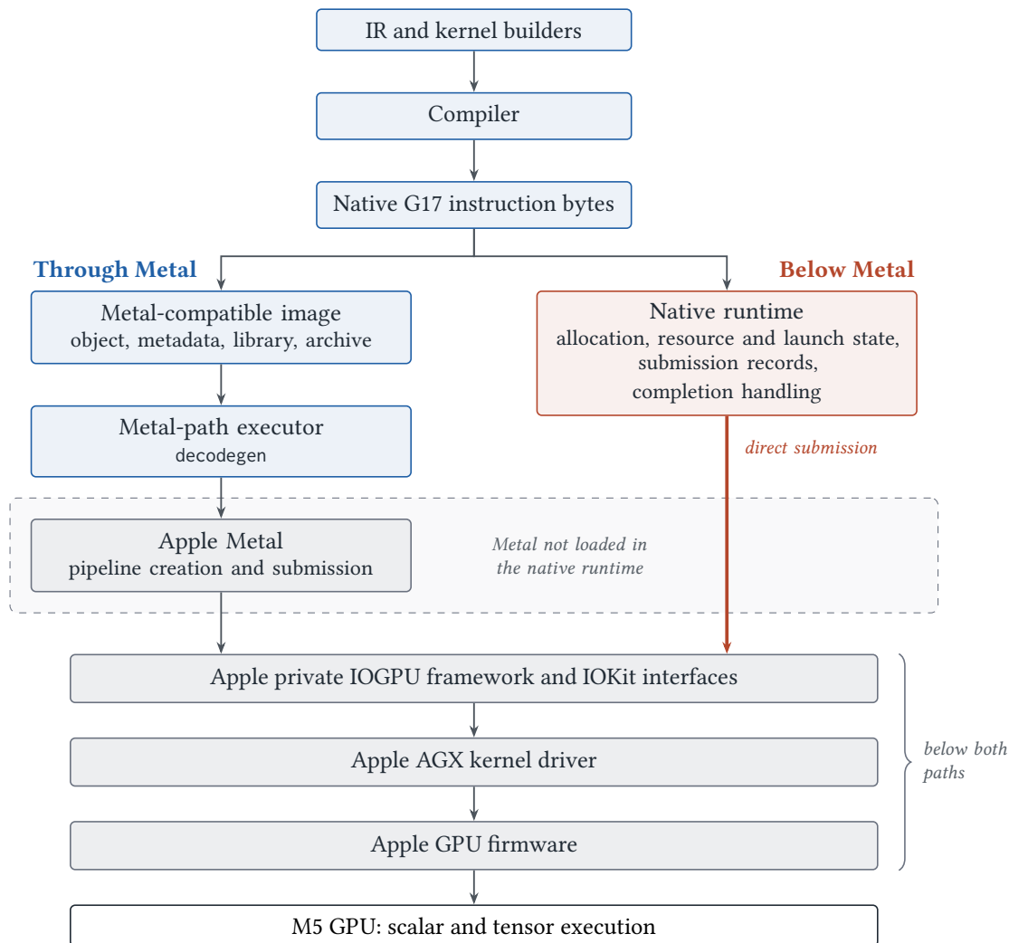
Figure 0.1. The two execution paths. The native runtime does its own pipeline setup and submits directly through IOGPU. Grey: Apple’s; blue: the project’s; red: the project’s native runtime.
