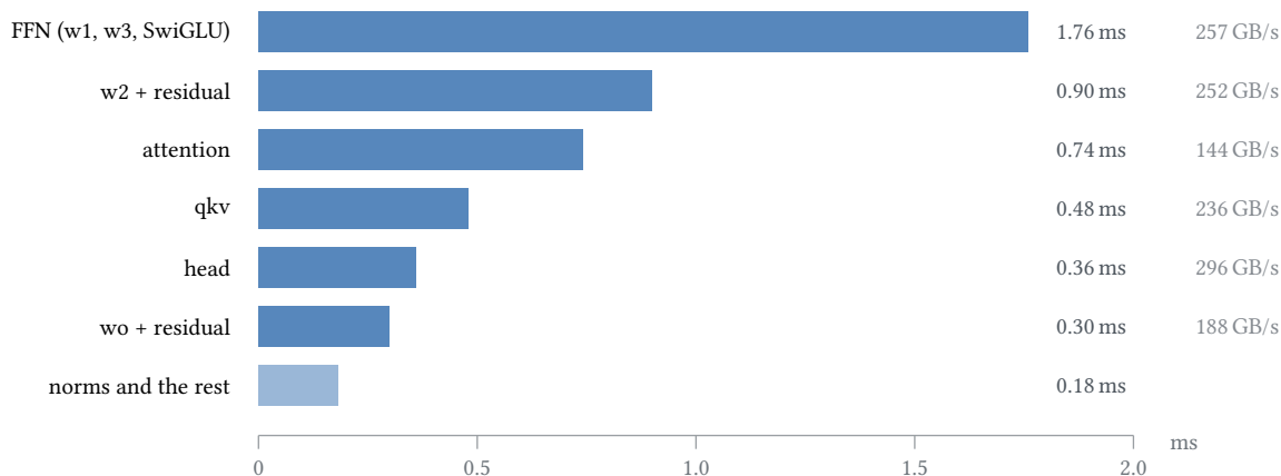
Figure 12.1. Where a token goes at a 1K context: 4.73 ms, by part and largest first, with the effective bandwidth each part reaches ( table 12.12 ). Only the head streams at the DRAM peak.
