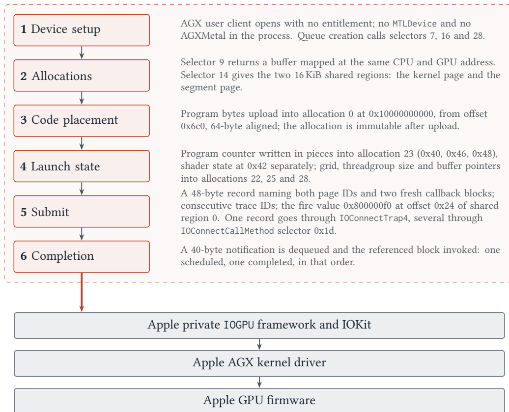
Figure 13.1. The below-Metal submission sequence. Every step inside the dashed box is written by the project’s runner; the bands below it stay Apple’s.
