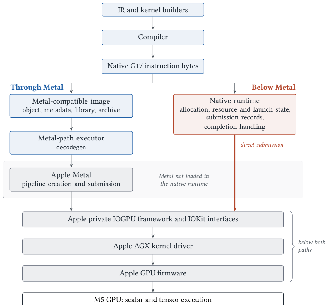
Figure 0.1. The two execution paths. The native runtime does its own pipeline setup and submits directly through IOGPU. Gray: Apple’s; blue: the project’s; red: the project’s native runtime.
