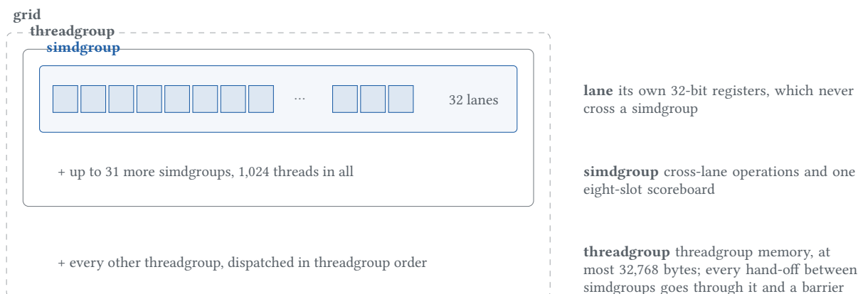
Figure 1.1. The execution hierarchy. SIMD width is 32 on every pipeline measured, and a threadgroup holds at most 1,024 threads.
