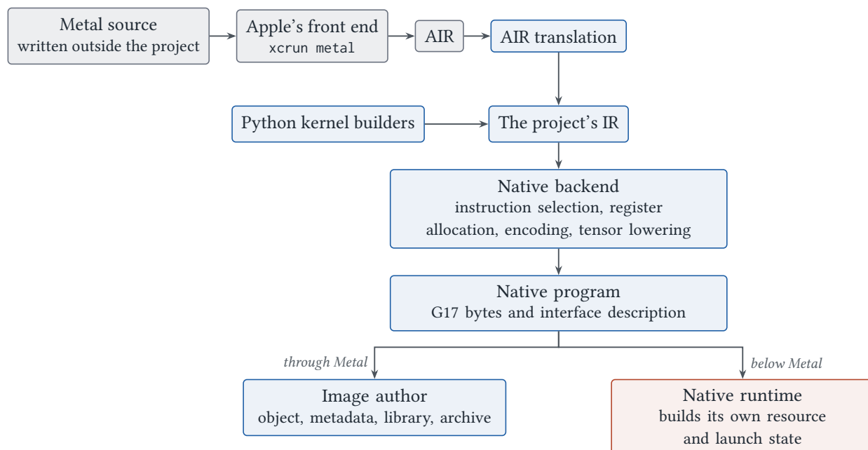
Figure 15.1. Input routes to a native program. Gray: Apple’s; blue: the project’s; red: the project’s native runtime.
