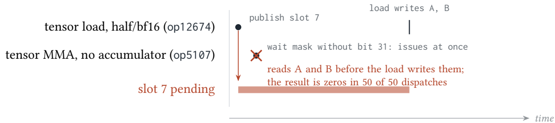
Figure 9.1. Late values and their waits, as the control words specify them. A dot is an instruction's issue; gray is an instruction held at issue by its wait mask; a colored bar is a scoreboard slot that a producer has published and whose value has not yet arrived. A dashed arrow is a slot's arrival releasing its waiter. The control words in (a) are read from the running example's bytes (the low 32 bits of operand 1: bits 20–23 publish slot + 1, bits 24–31 are the wait mask). Panel (b) is the measured missing-wait experiment. Positions on the time axis are schematic; only the order is measured.
