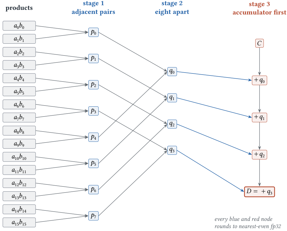
Figure 10.3. The measured reduction of one output element. One 16 \times 16 \times 16 MMA computes each output element from sixteen exact products. Stage 1 adds adjacent products, p_i = \text{RNE}_{32}(a_{2i}b_{2i} + a_{2i+1}b_{2i+1}) ; stage 2 adds partial sums eight products apart, q_i = \text{RNE}_{32}(p_i + p_{i+4}) ; stage 3 starts from the accumulator C and adds q_0, \dots, q_3 in order, rounding at every step. The from-zero form, tensor MMA, 16-bit \times 16-bit, no accumulator (op5107), has no C and starts the chain from q_0 . The diagram shows data dependence and makes no claim about the physical addresses (MM 4, MM 0.6).
