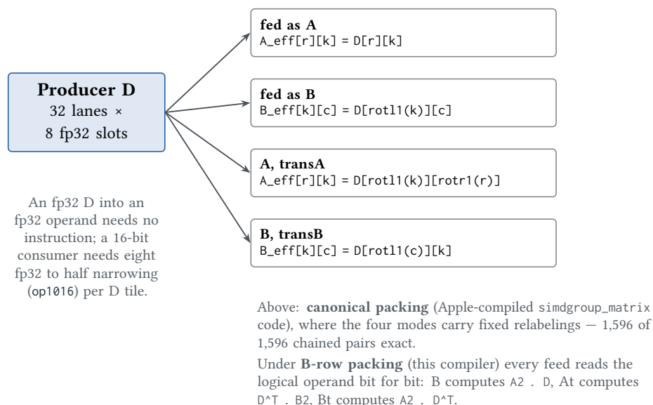
Figure 10.5. The four feed modes of a register-direct chain. The direct chain is bit-identical to the memory bridge on 200 of 200 random matrices; which relabeling applies depends on how the producing kernel packed its tiles, not on the instruction.
