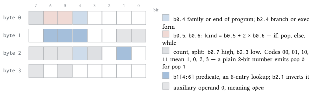
Figure 5.1. The word the exec-mask family and the branches share. Every field but the auxiliary operand is established; hard-coding one value per kind for that operand writes an instruction Apple never emitted for 5.66 percent of its 14,195 control-flow instructions, and hard-coding zero for 19.38 percent ( table 5.1 ).
