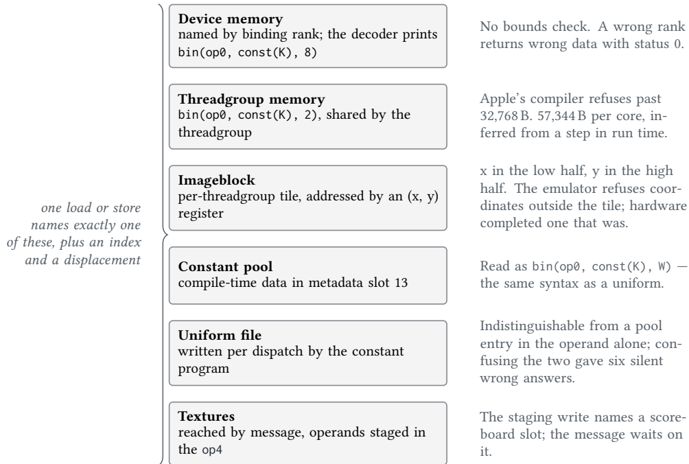
Figure 7.1. Where an access can point. The opcode fixes the element width; there is no width field, and the hardware checks neither the bound nor whether a loaded value has arrived.
