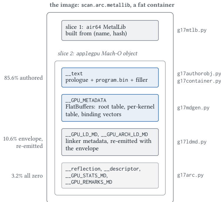
Figure 11.1. The delivered image, outside in, with the tool that authors each layer on the right and the census share of table 11.4 on the left. Blue: bytes the project authors; gray: the envelope it re-emits from the object and the entry name.
