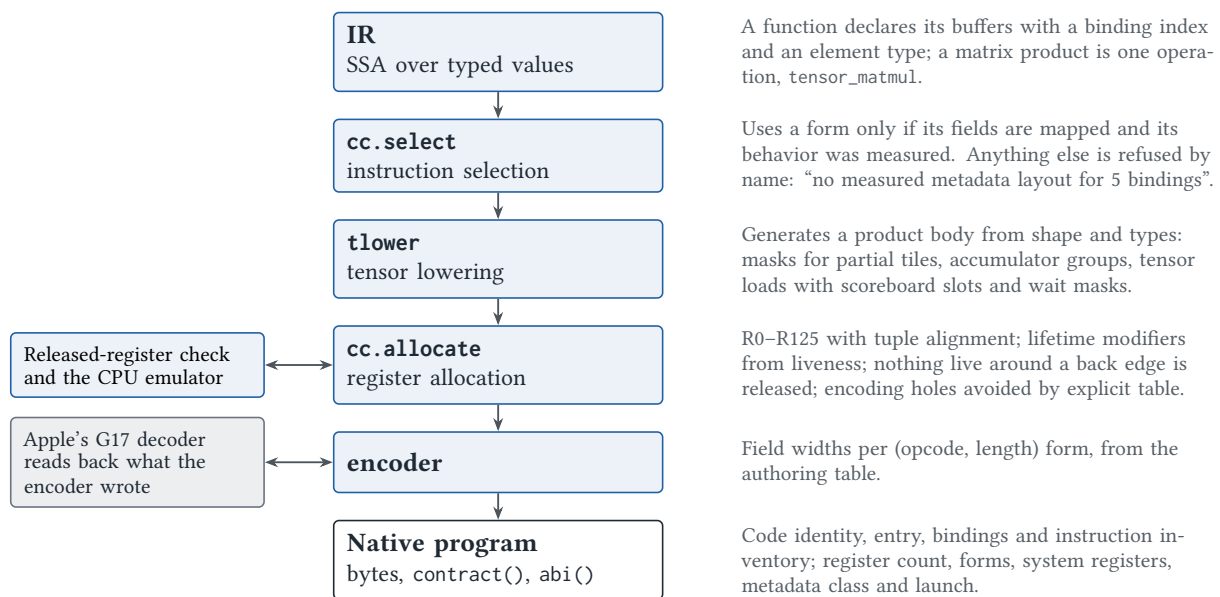
Figure 15.2. Inside the backend. Each stage refuses what it cannot justify rather than guessing, and every compile decodes its own output with Apple’s decoder.
