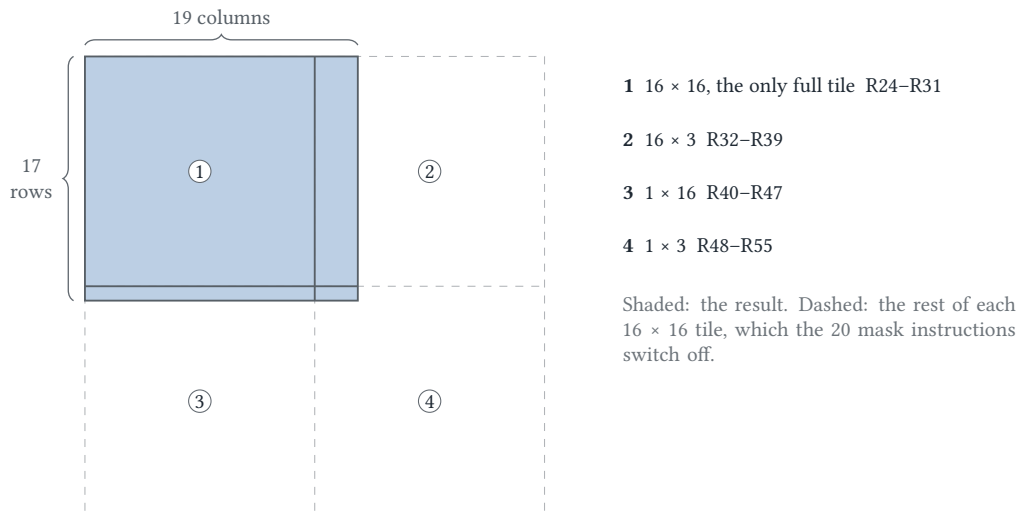
Figure 0.2. The running example's output against the tiles that cover it. A 17 \times 19 result does not divide into 16 \times 16 , so it takes two tile rows by two tile columns, three of them partial: one tensor MMA, 16-bit \times 16-bit, no accumulator (op5107) and one eight-register accumulator group each.
