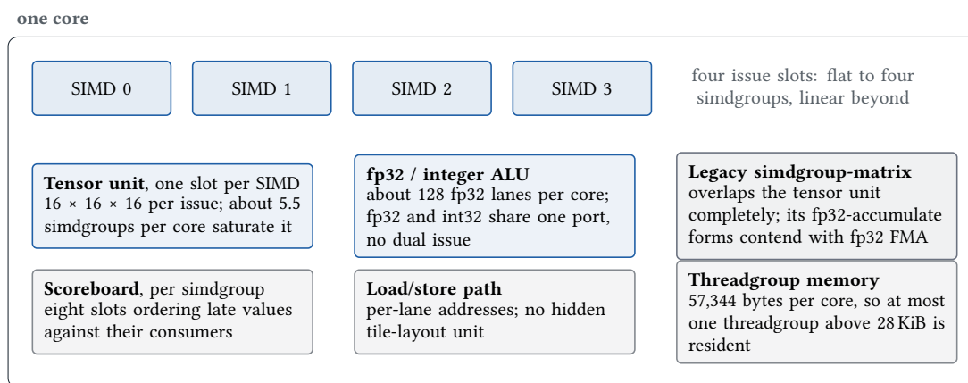
Figure 1.2. One core, as measured concurrency describes it: which streams run beside each other and which contend. This is a logical account and does not locate or count physical units ( table 1.2 ).
