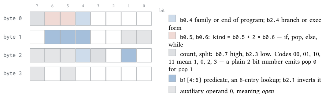
Figure 5.1. The word the exec-mask family and the branches share. Every field but the auxiliary operand is established; hard-coding one value per kind for that operand writes an instruction Apple never emitted for 5.66 percent of its 14,195 control-flow instructions, and hard-coding zero for 19.38 percent ( table 5.1 ).
