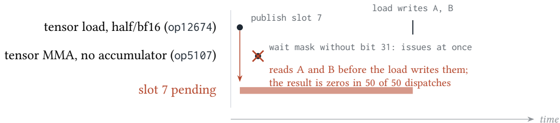
Figure 9.1. Late values and their waits, as the control words specify them. A dot is an instruction's issue; grey is an instruction held at issue by its wait mask; a coloured bar is a scoreboard slot that a producer has published and whose value has not yet arrived. A dashed arrow is a slot's arrival releasing its waiter. The control words in (a) are read from the running example's bytes (the low 32 bits of operand 1: bits 20–23 publish slot + 1, bits 24–31 are the wait mask). Panel (b) is the measured missing-wait experiment. Positions on the time axis are schematic; only the order is measured.
