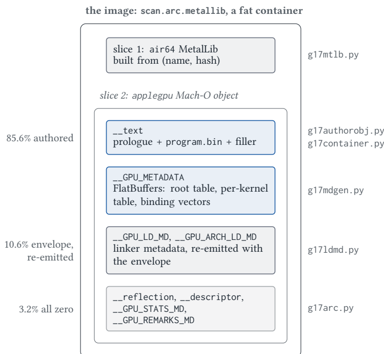
Figure 11.1. The delivered image, outside in, with the tool that authors each layer on the right and the census share of table 11.4 on the left. Blue: bytes the project authors; grey: the envelope it re-emits from the object and the entry name.
