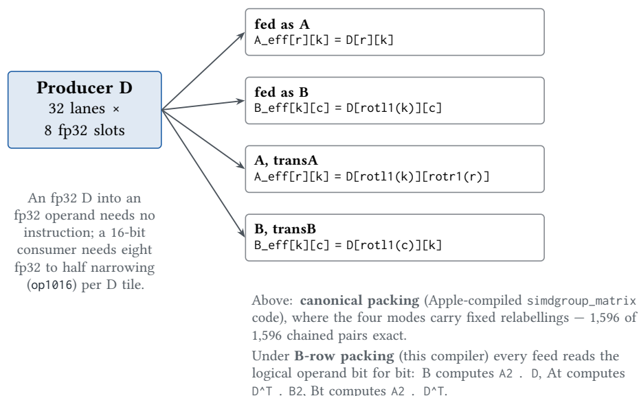
Figure 10.5. The four feed modes of a register-direct chain. The direct chain is bit-identical to the memory bridge on 200 of 200 random matrices; which relabelling applies depends on how the producing kernel packed its tiles, not on the instruction.
