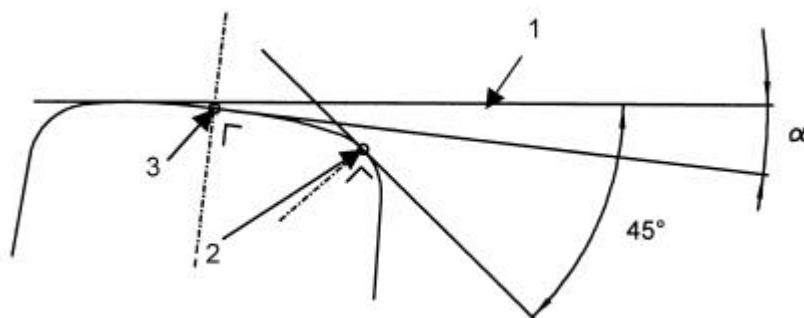
(b) Detailed section of railhead, showing reference point A and B'. ( \alpha :angle of rail inclination)
