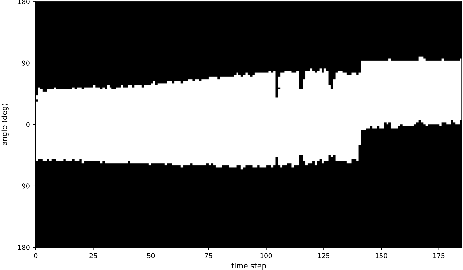
Run 43 | Seed 1548504369
