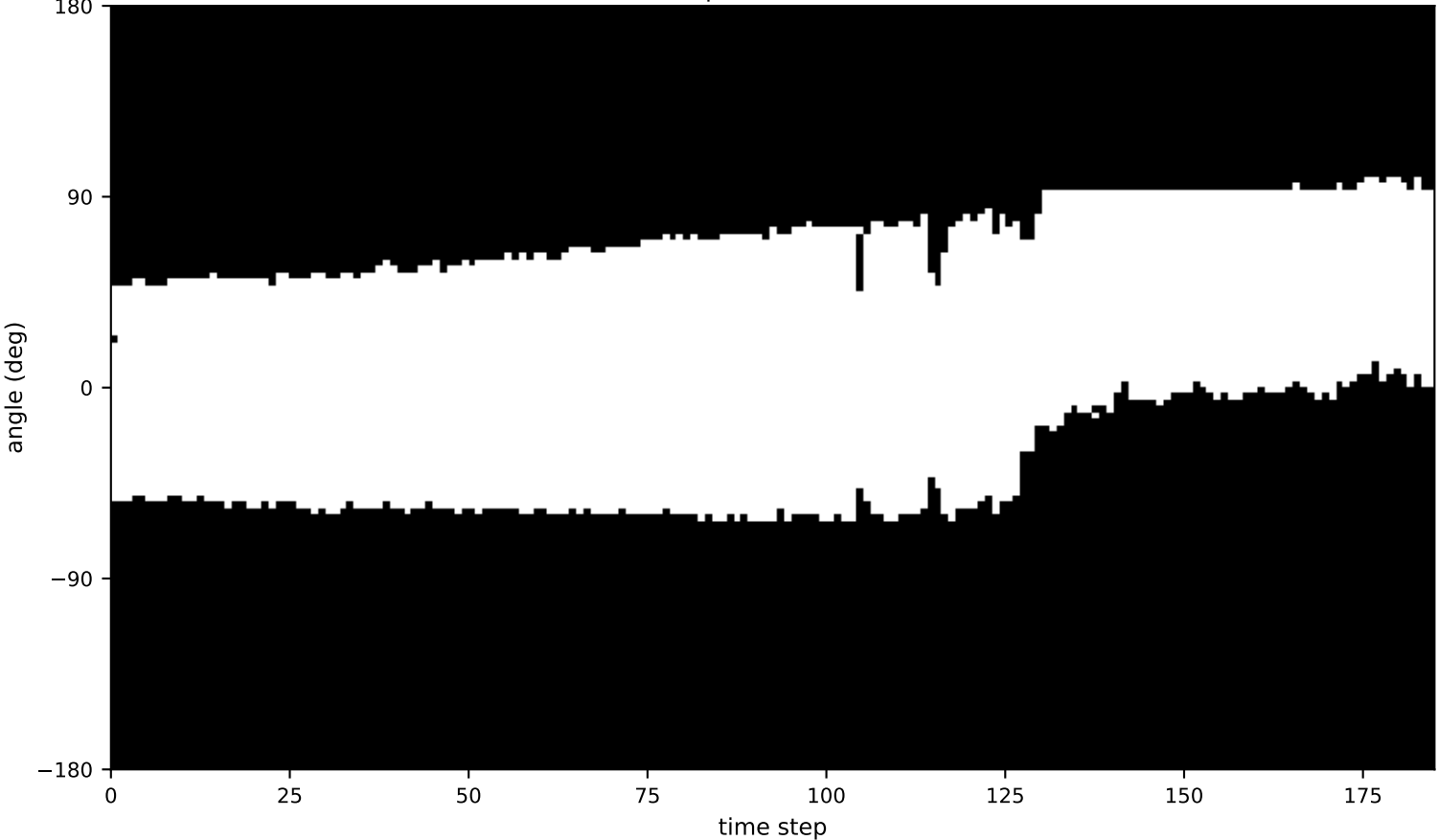
Run 44 | Seed 577726471
