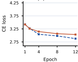
(a) B = 16
