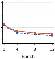
(b) B = 64
