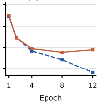
(c) B = 512
