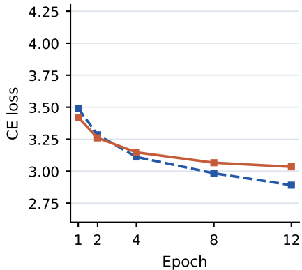
(a) B = 16
