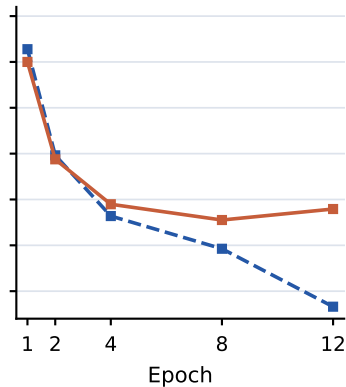
(c) B = 512
