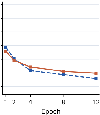
(b) B = 64
