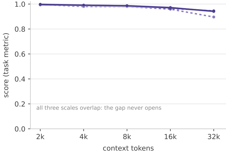
(a) HotpotQA
