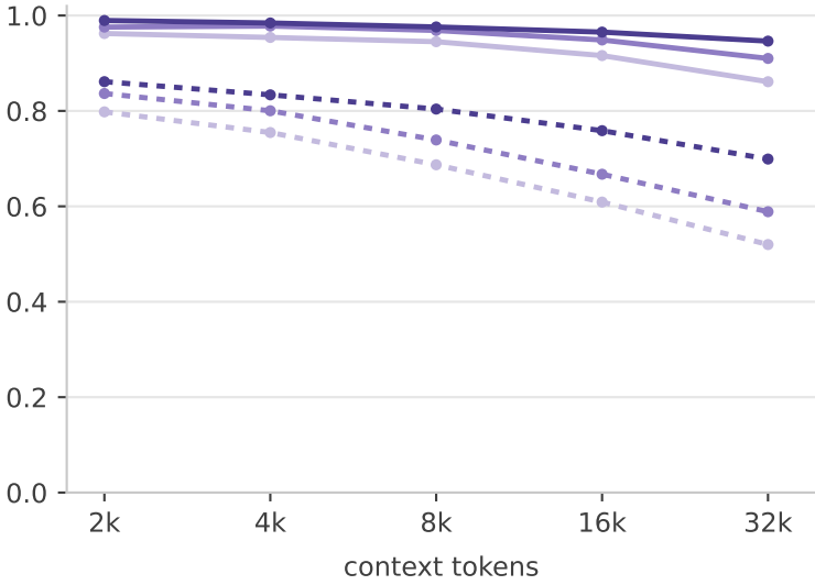
(c) contradiction
