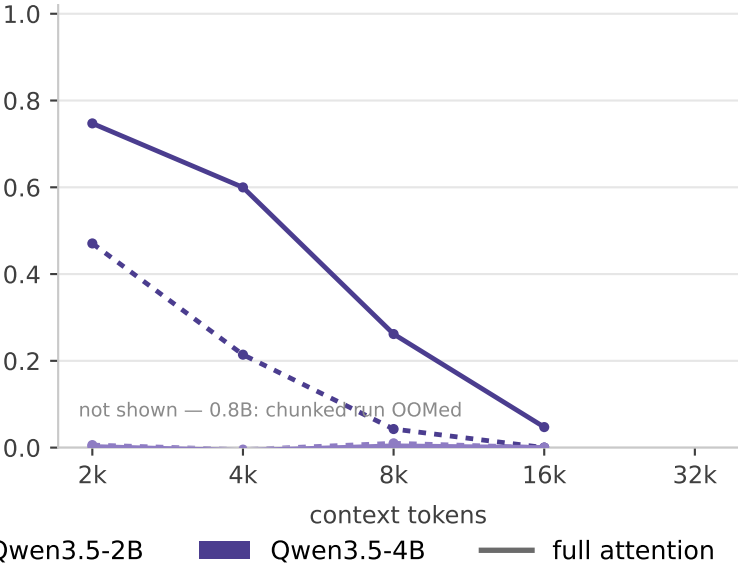
(e) reordering
