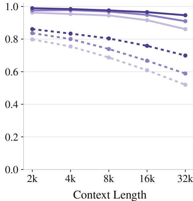
Contradiction
