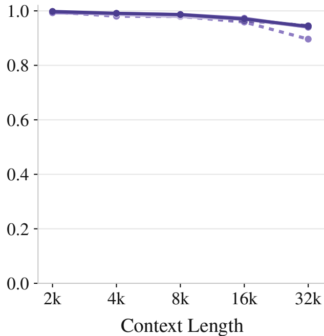
HotpotQA
