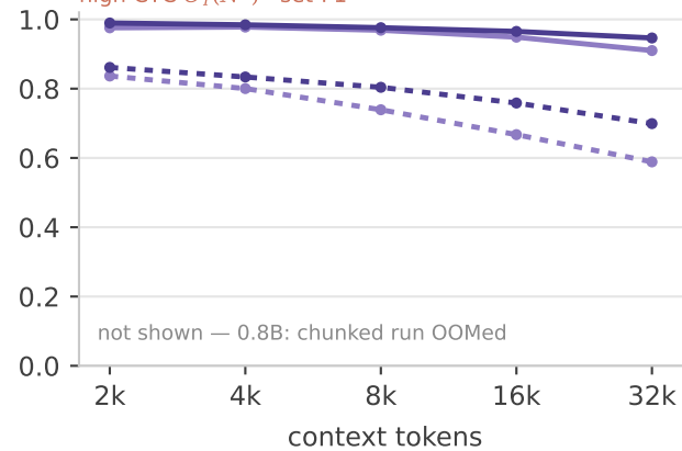
(c) contradiction
