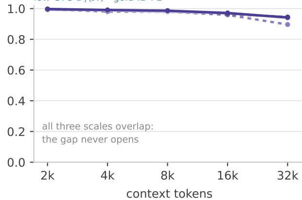
(a) HotpotQA
