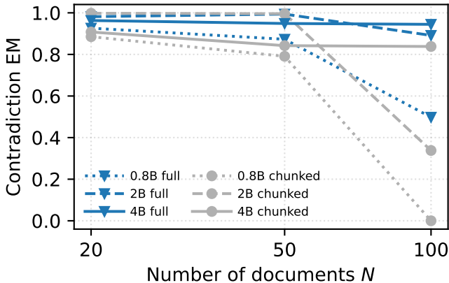
Qwen-3.5 model scale (full vs chunked)
