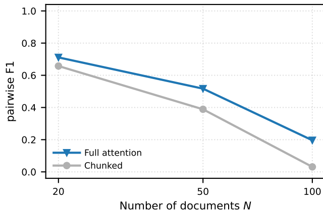
Grouping (OpenAlex, Qwen3.5-4B)
