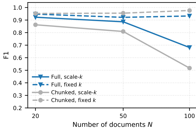
Outlier (wiki, Qwen3.5-4B)
