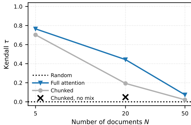
Reorder (Gutenberg, Qwen3.5-9B)
