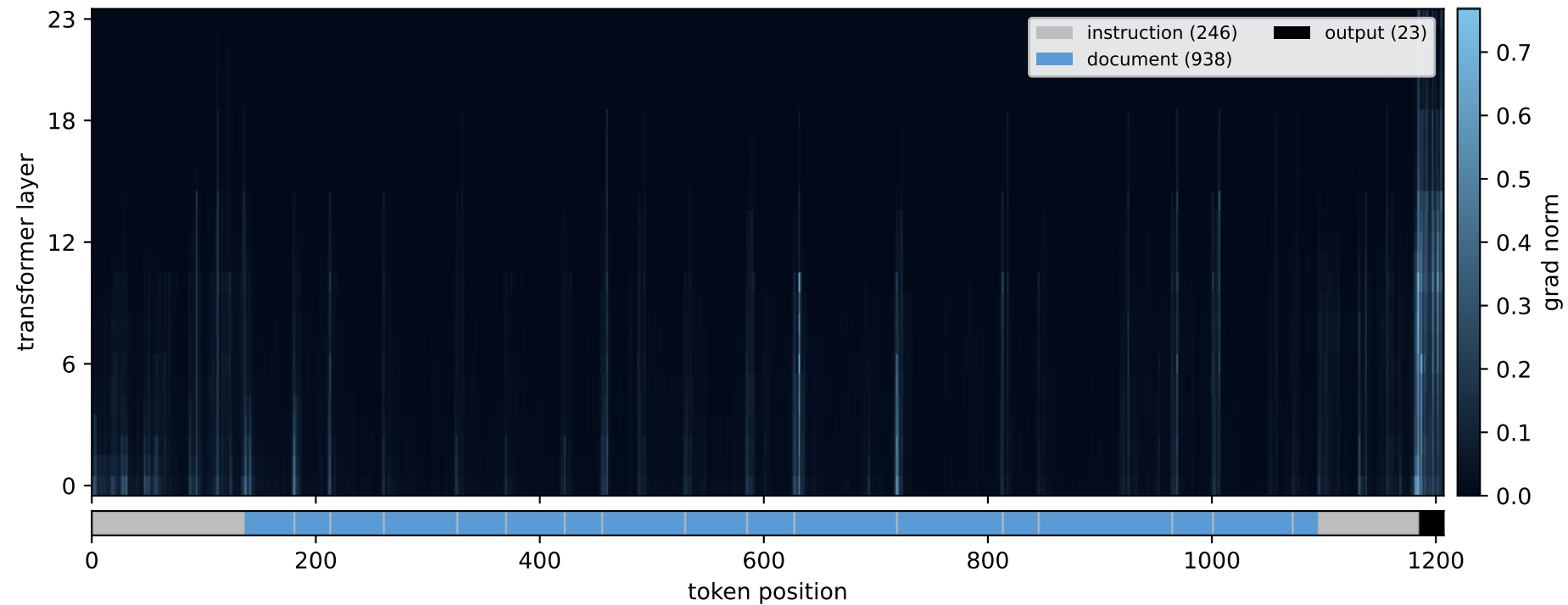
Per-token, per-layer gradient L2 norm — contradiction (N=20, no CoT, full attention), 1207 tokens, loss 0.92
