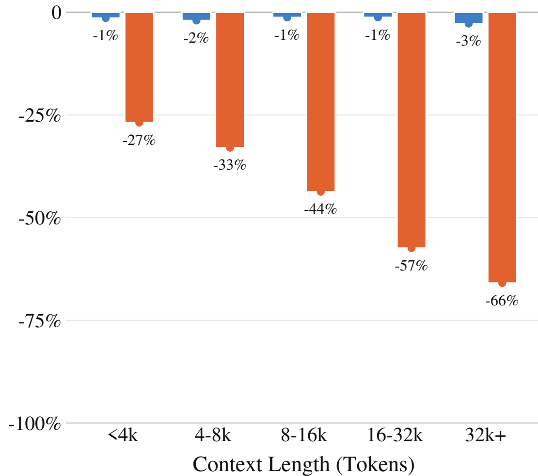
Performance Drop vs. Full Attention
