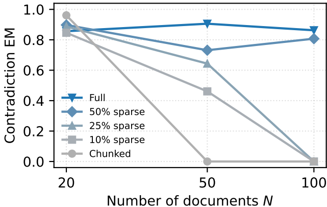
Qwen-2.5-3B, varying attention sparsity
