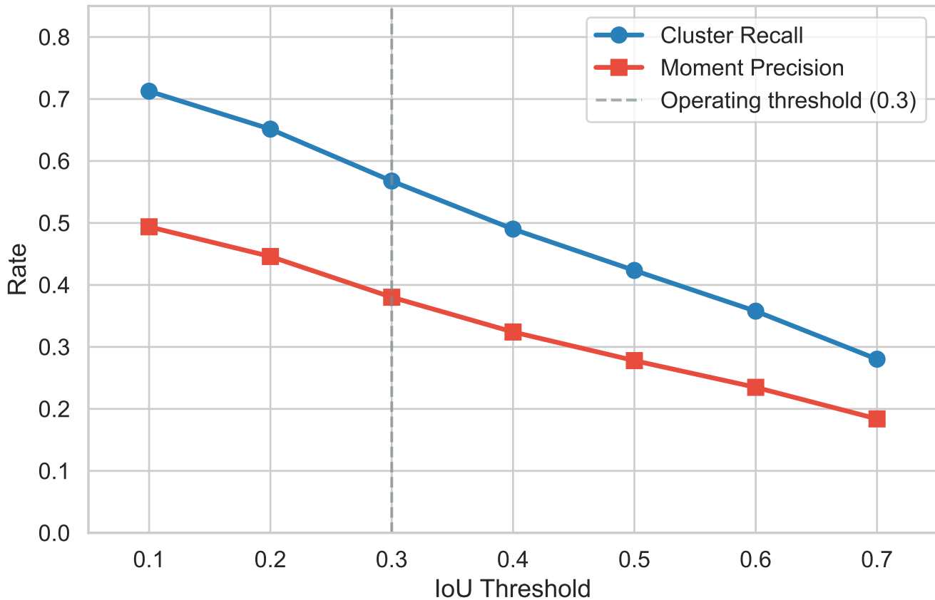
v5 Detection Performance vs. IoU Threshold (n=195 conversations)
