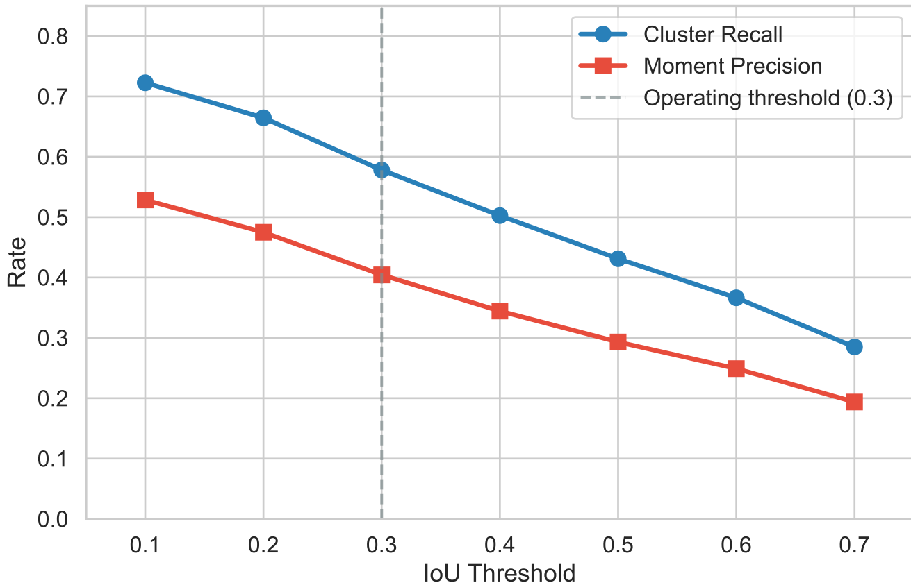
v5 Detection Performance vs. IoU Threshold (n=193 conversations)
