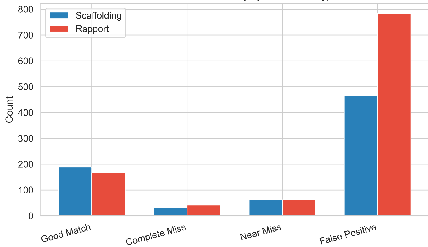
Detection Error Taxonomy by Annotation Type
