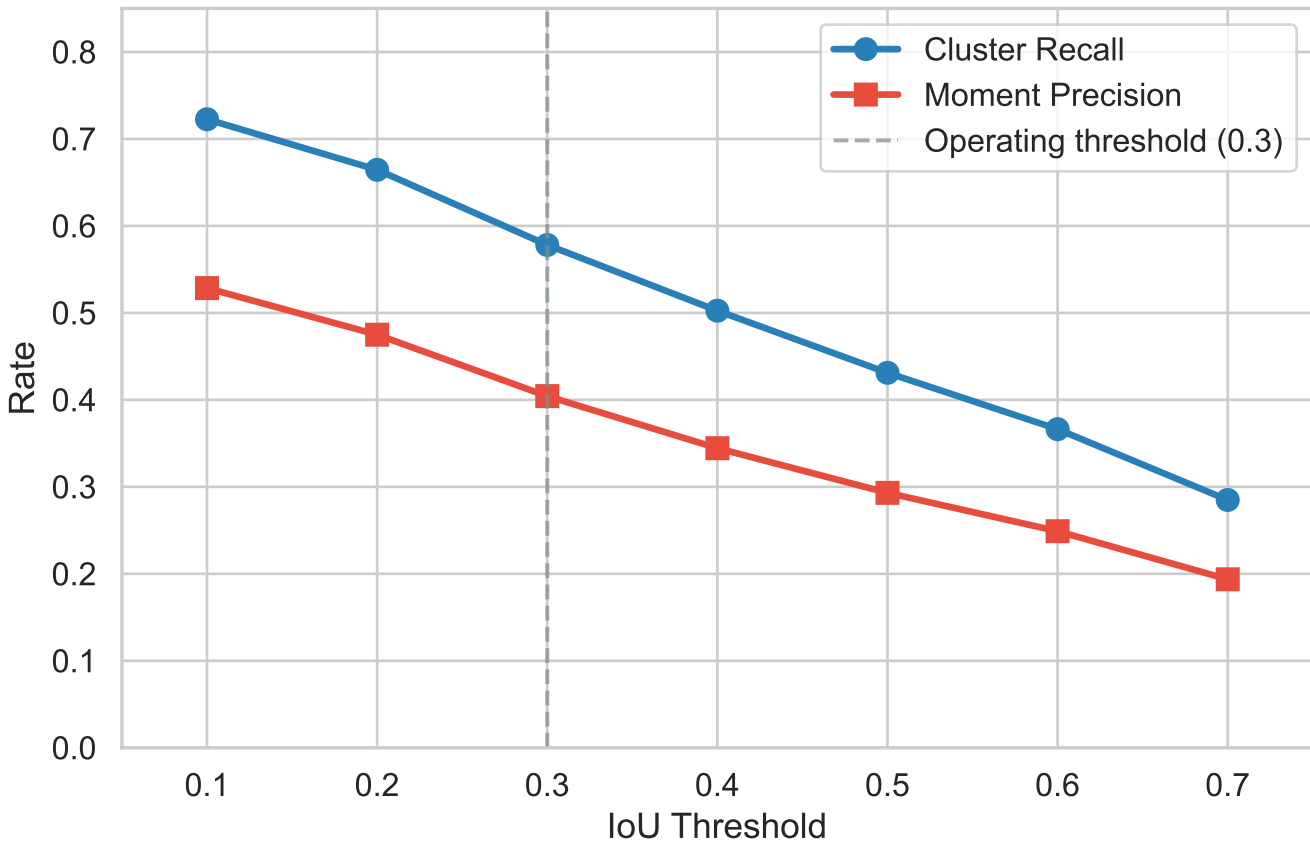
Detection Performance vs. IoU Threshold (n=193 conversations)
