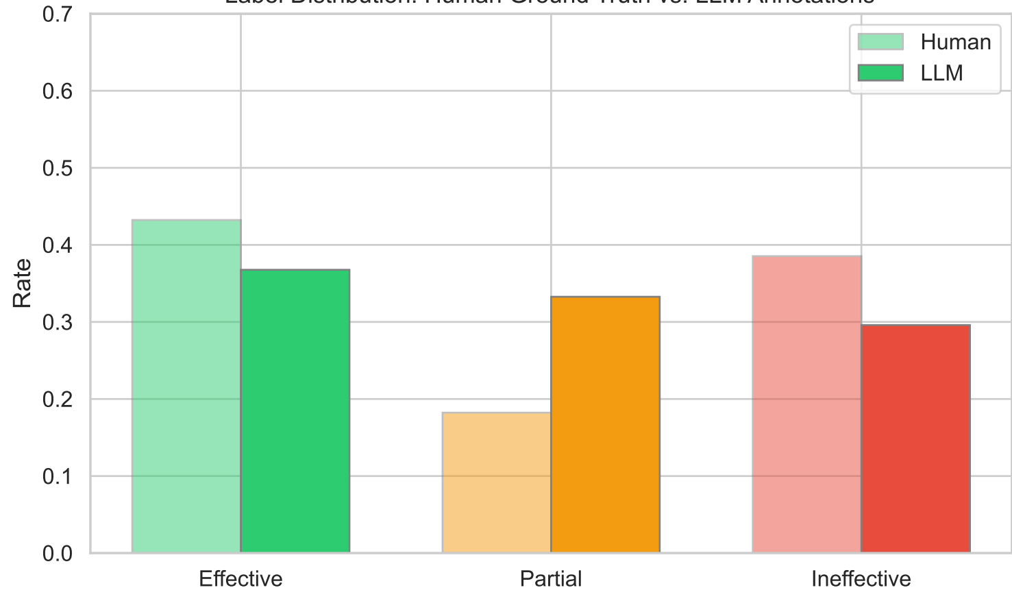
Label Distribution: Human Ground Truth vs. LLM Annotations
