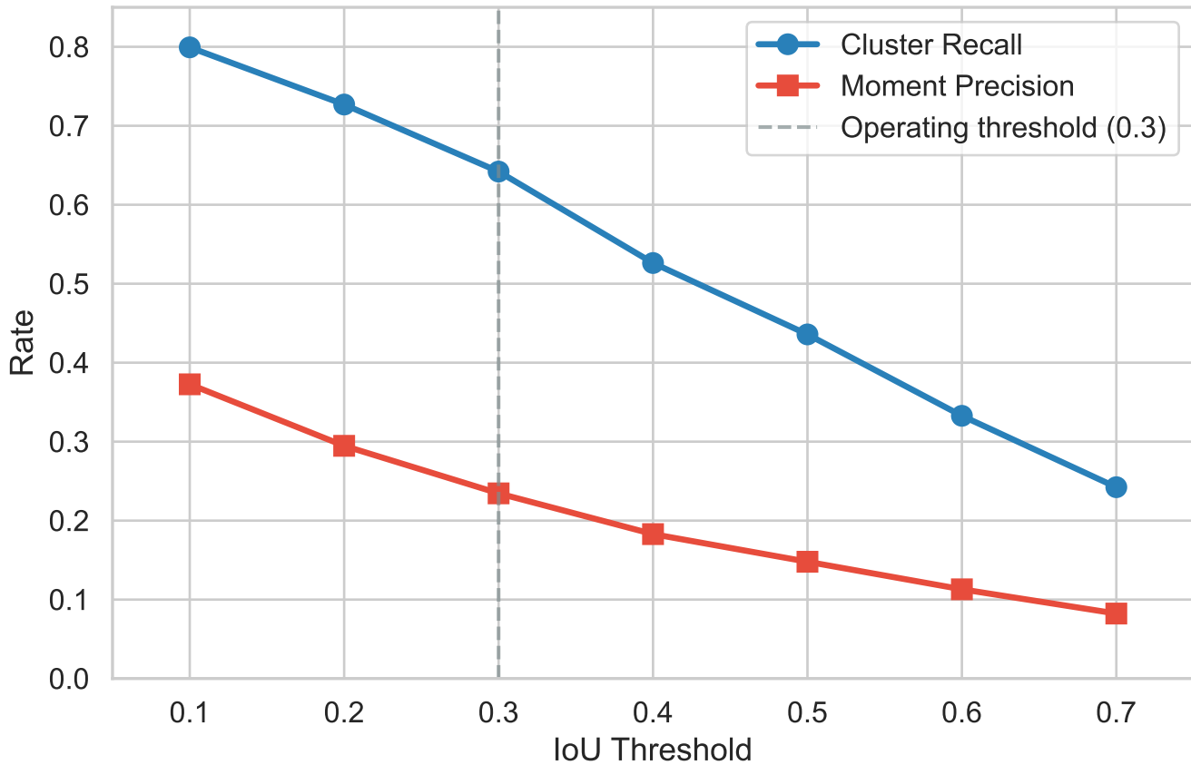
Detection Performance vs. IoU Threshold
