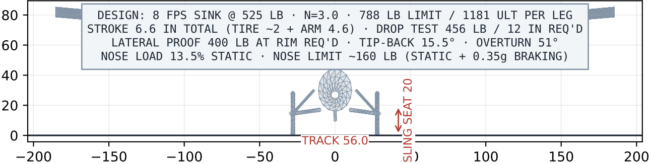
FRONT — TRACK AND STANCE
