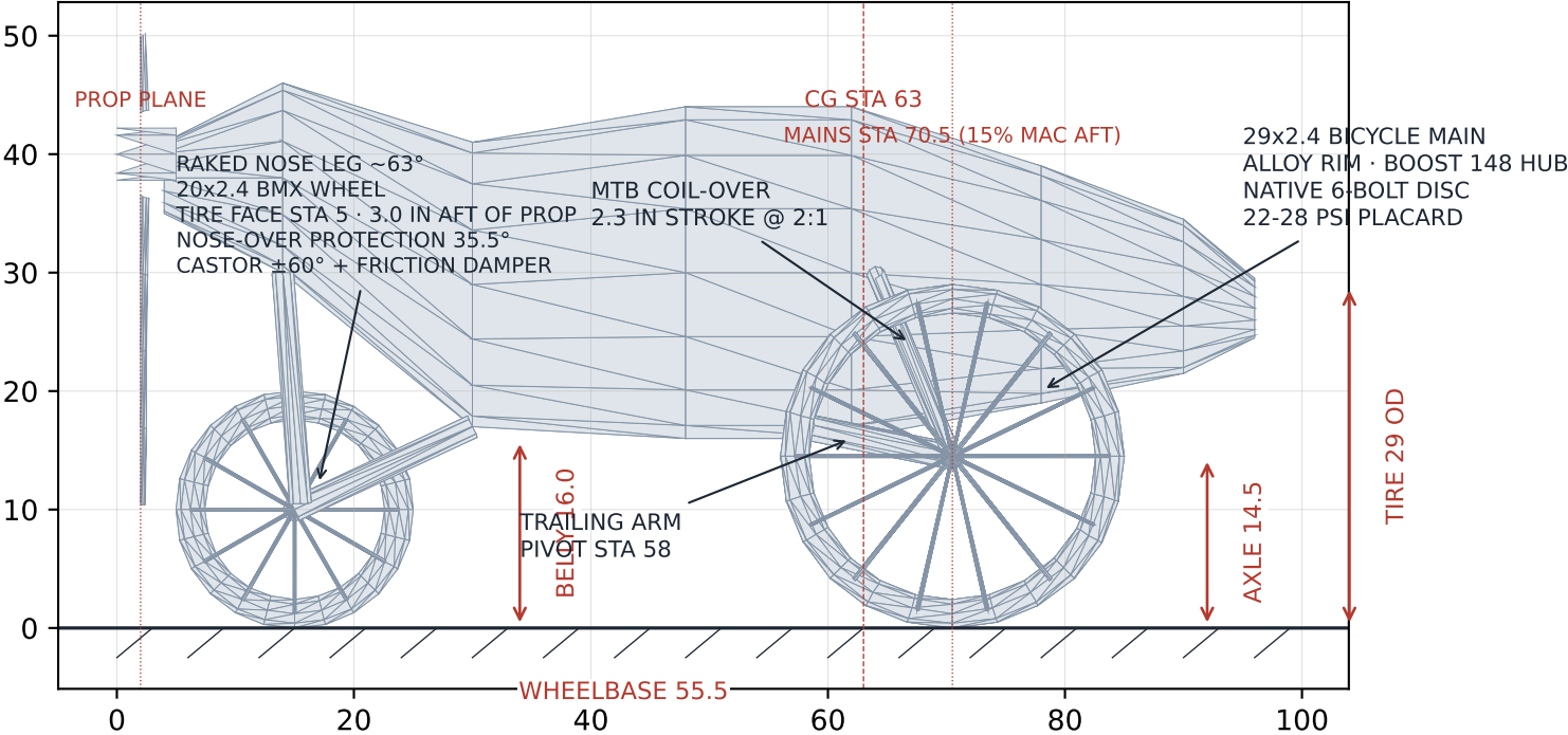
SIDE — TRAILING ARM MAIN GEAR
