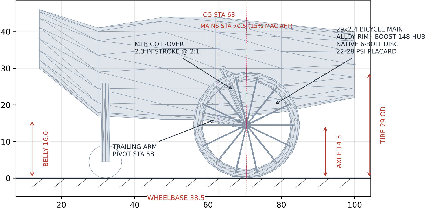
SIDE — TRAILING ARM MAIN GEAR
