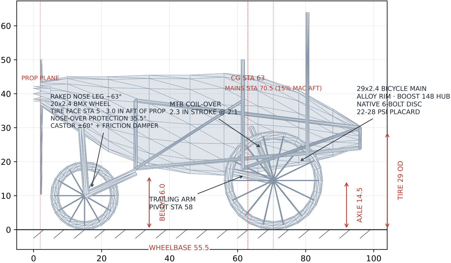
SIDE — TRAILING ARM MAIN GEAR
