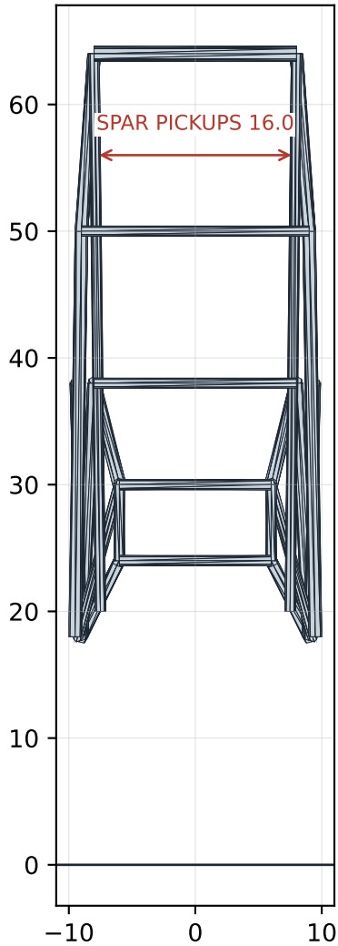
FRONT — CAGE SECTION
